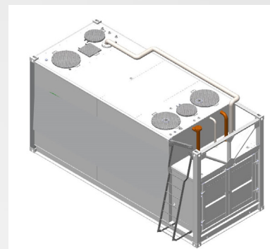
Dual Diesel and insulated DEF chemical resistant tanks
